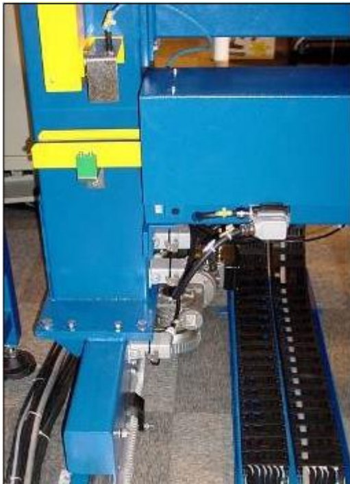
Sword including sword case on lateral sled including energy chains. Rack and pinion drive for accurate Positioning of the machine
